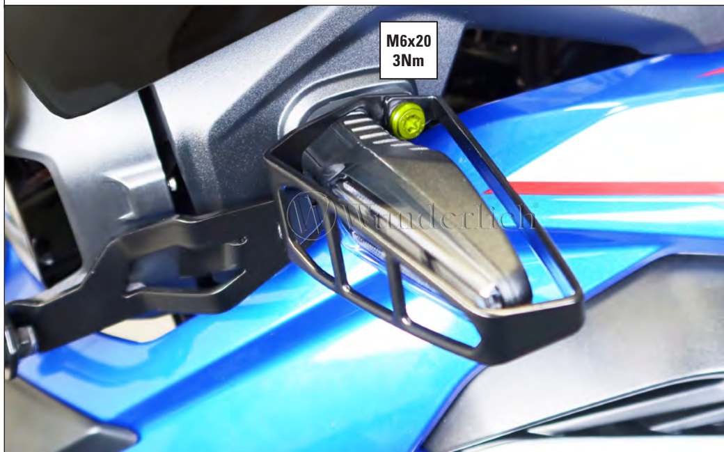
Art.-Nr: 42841-602 /-802 kurze Blinkervariante short indicator version
